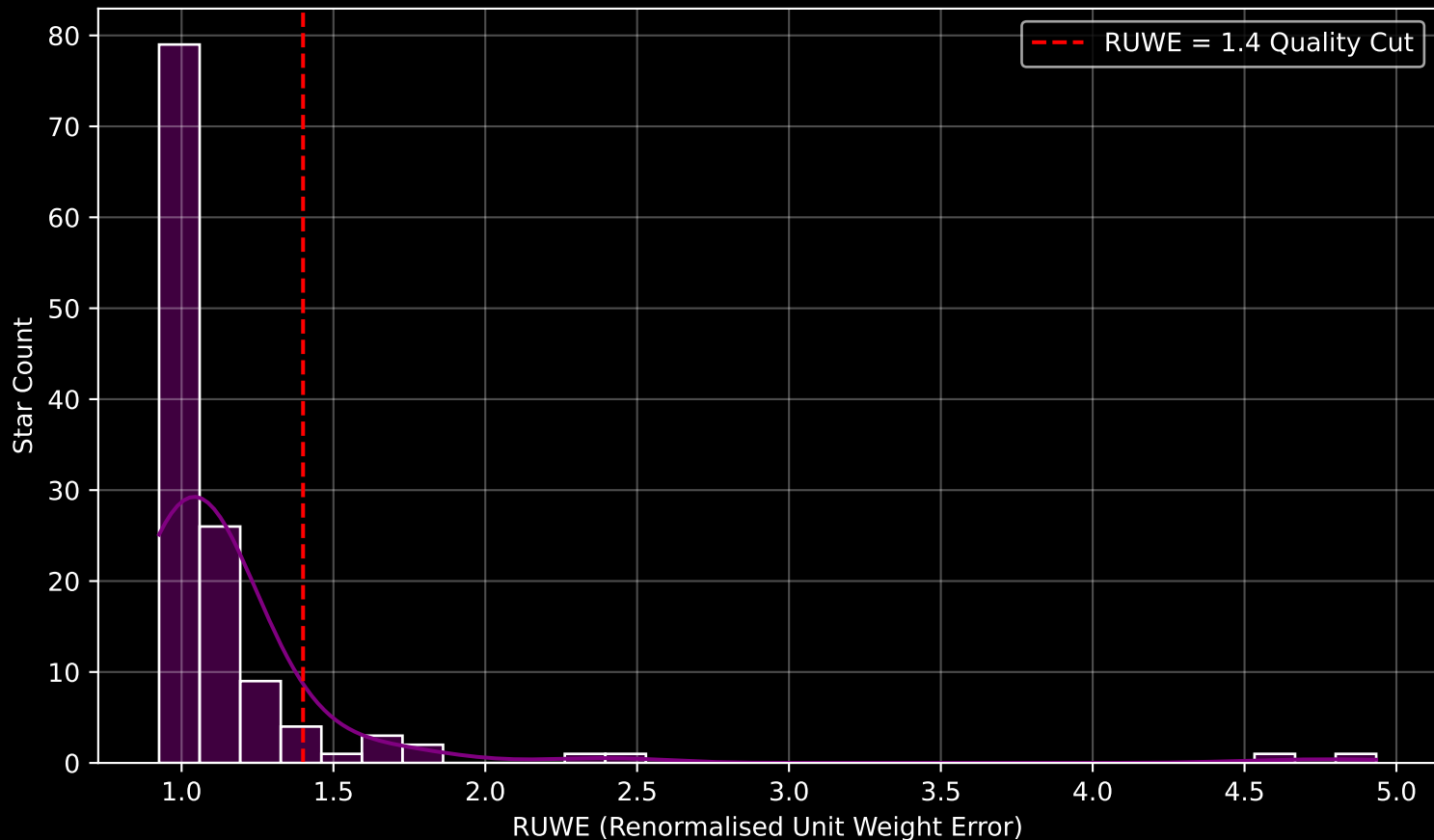
GAPOGEE DR17 Field [090-12] RUWE Distribution (n= 128)
