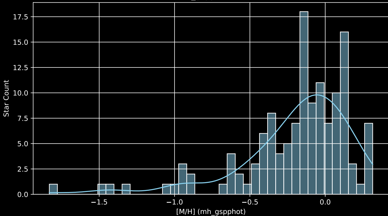
APOGEE DR17 Field: [090-12 [M/H] (mh_gspphot) (n= 134)
