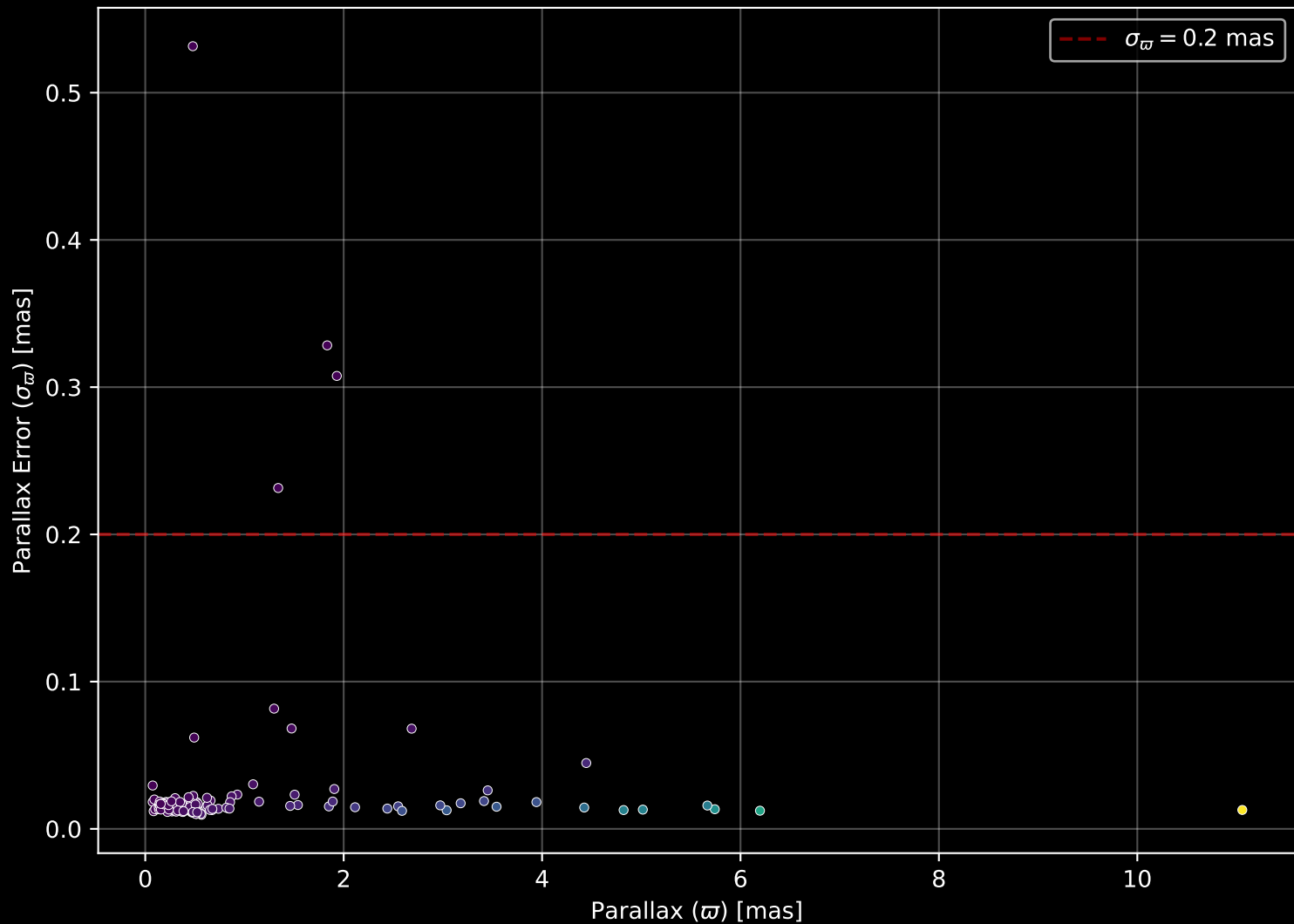
APOGEE DR17 Field: [090-12] Parallax Quality (n= 134)
