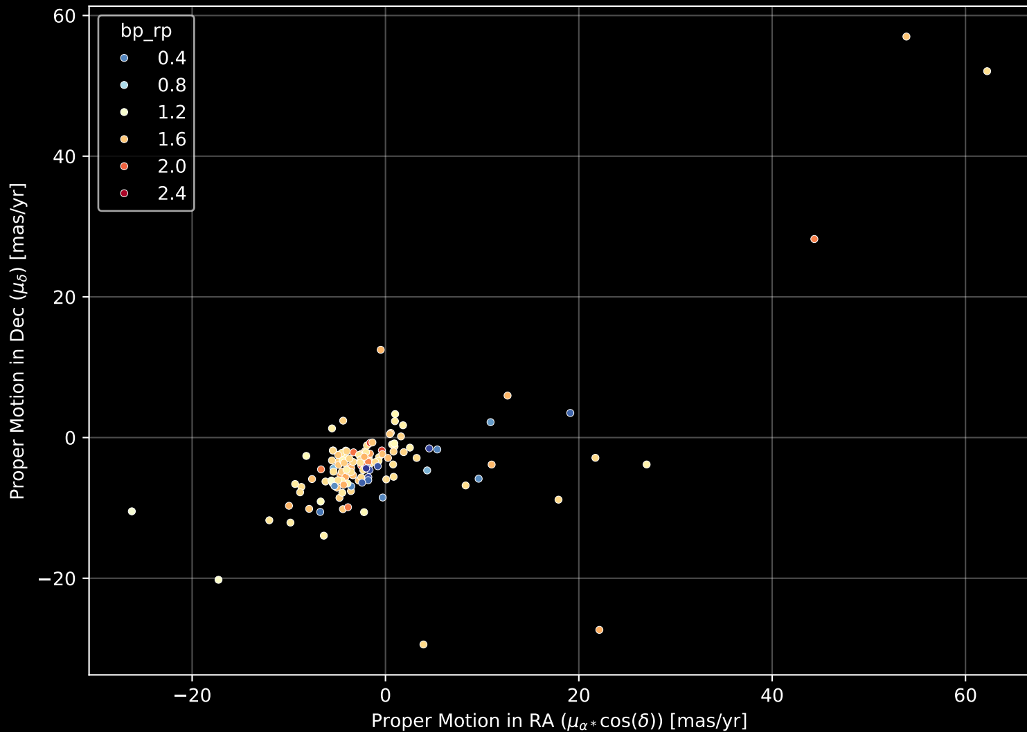
APOGEE DR17 Field: [090-12] Proper Motion Diagram (n= 134)
