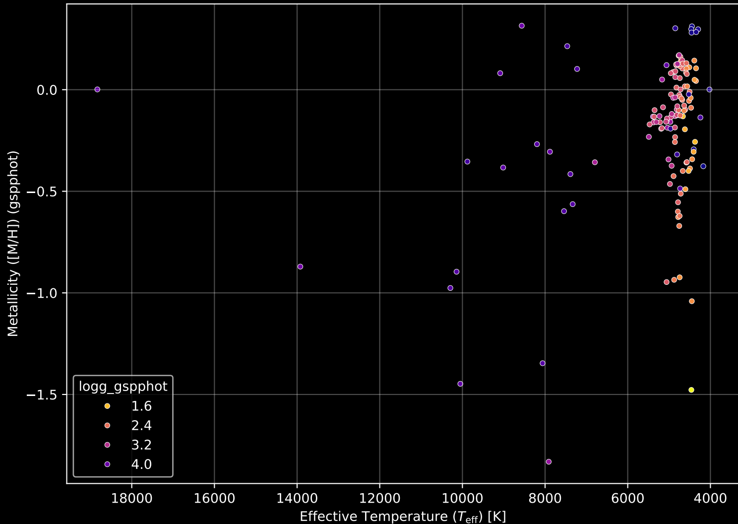
APOGEE DR17 Field: [090-12] Stellar Population Parameters (n= 134)
